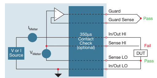
Contact check option for 4-wire or 6-wire applications
